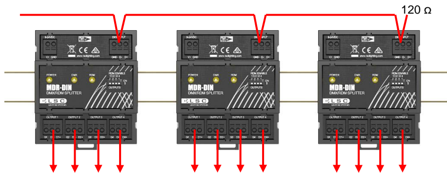
Recommended method of cascading multiple MDRD/T splitters
