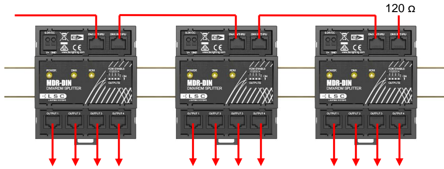
Recommended method of cascading multiple MDRD/J splitters
